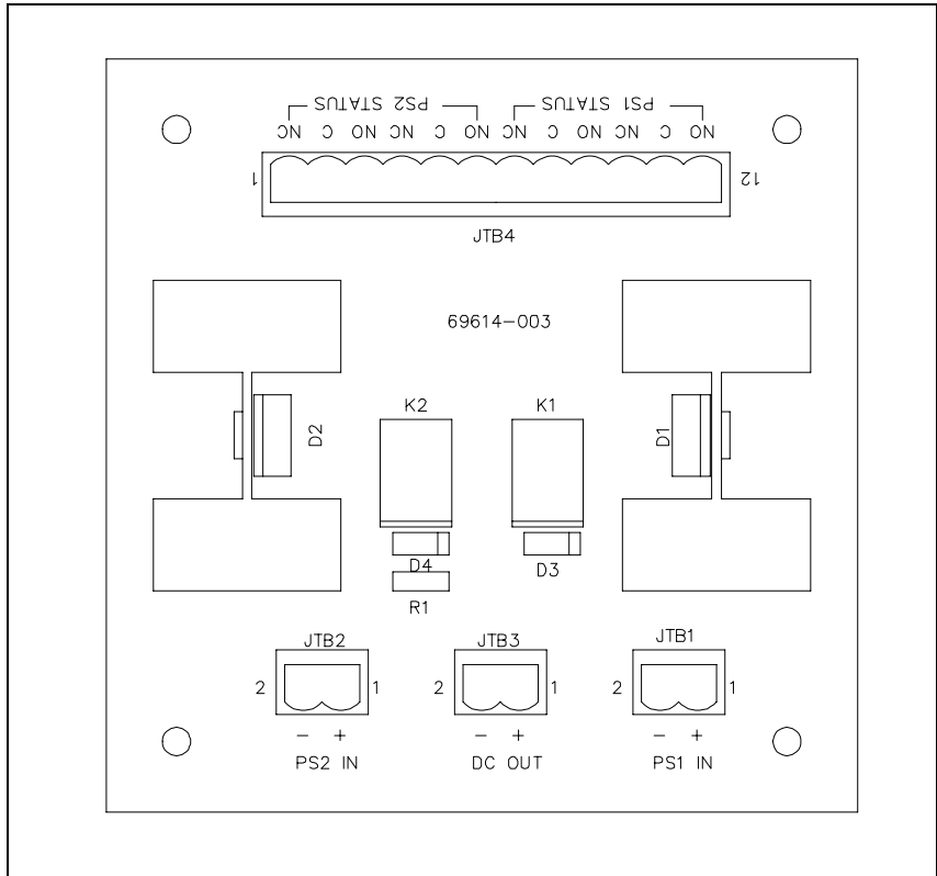
Figure 1. Model 12598-003 Redundant 24 V DC Module
